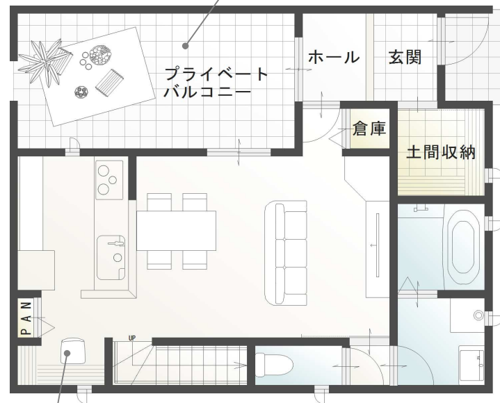
PLAN VIEW 1F
