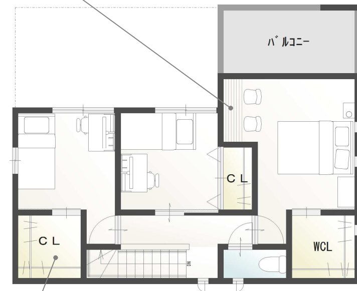
PLAN VIEW 2F
