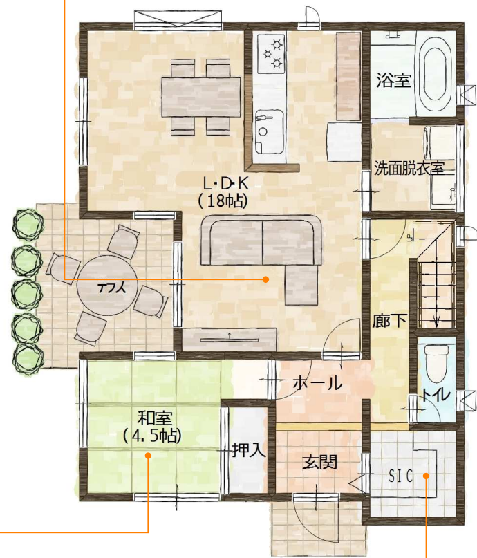
Plan View 1f
